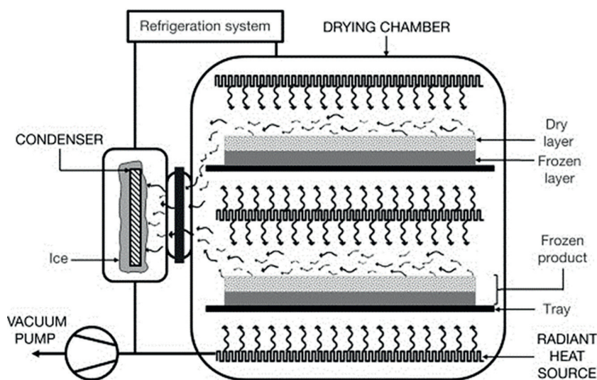
Figure 5. Freeze-drying process.
