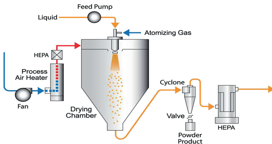
Figure 6. Spray drying process.
